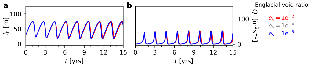
Figure D1. Lake water height, l_h (left panel, a) and sum discharge at the ice–lake contact, Q_r (right panel, b) for the englacial void ratio e_v parameter in our synthetic experiments. In each panel, the reference parameter experiment (Section 3) is shown in grey.
