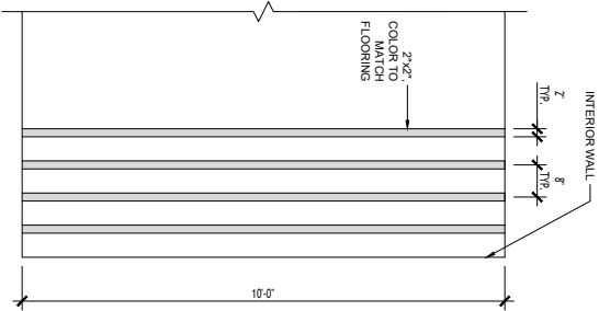
2 WOOD SLAT DETAIL @ WALL SCALE: 3/4" = 1'-0"
