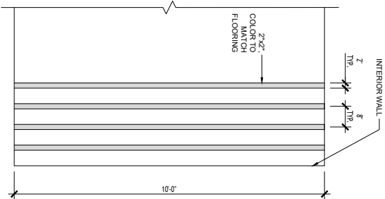
2 WOOD SLAT DETAIL @ WALL SCALE: 3/4" = 1'-0"
