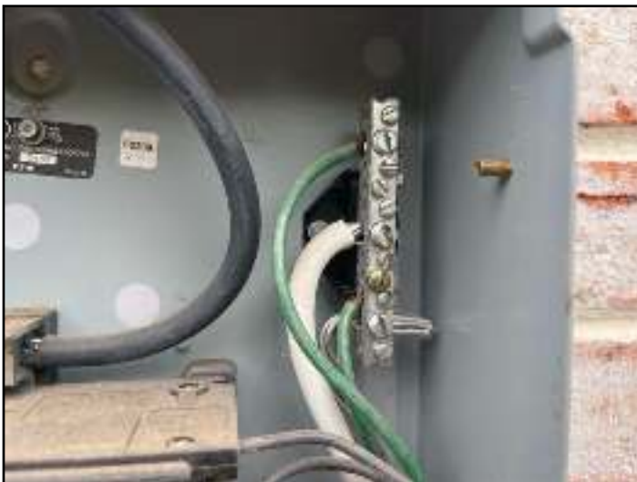
77. Neutral and ground wires bonded at auxiliar...
