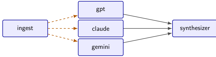
Figure 3: Fan-out / fan-in with multi-model ensembling.
