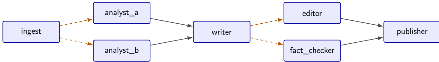
Figure 6: Compound pattern combining fan-in, fan-out, and final aggregation.
