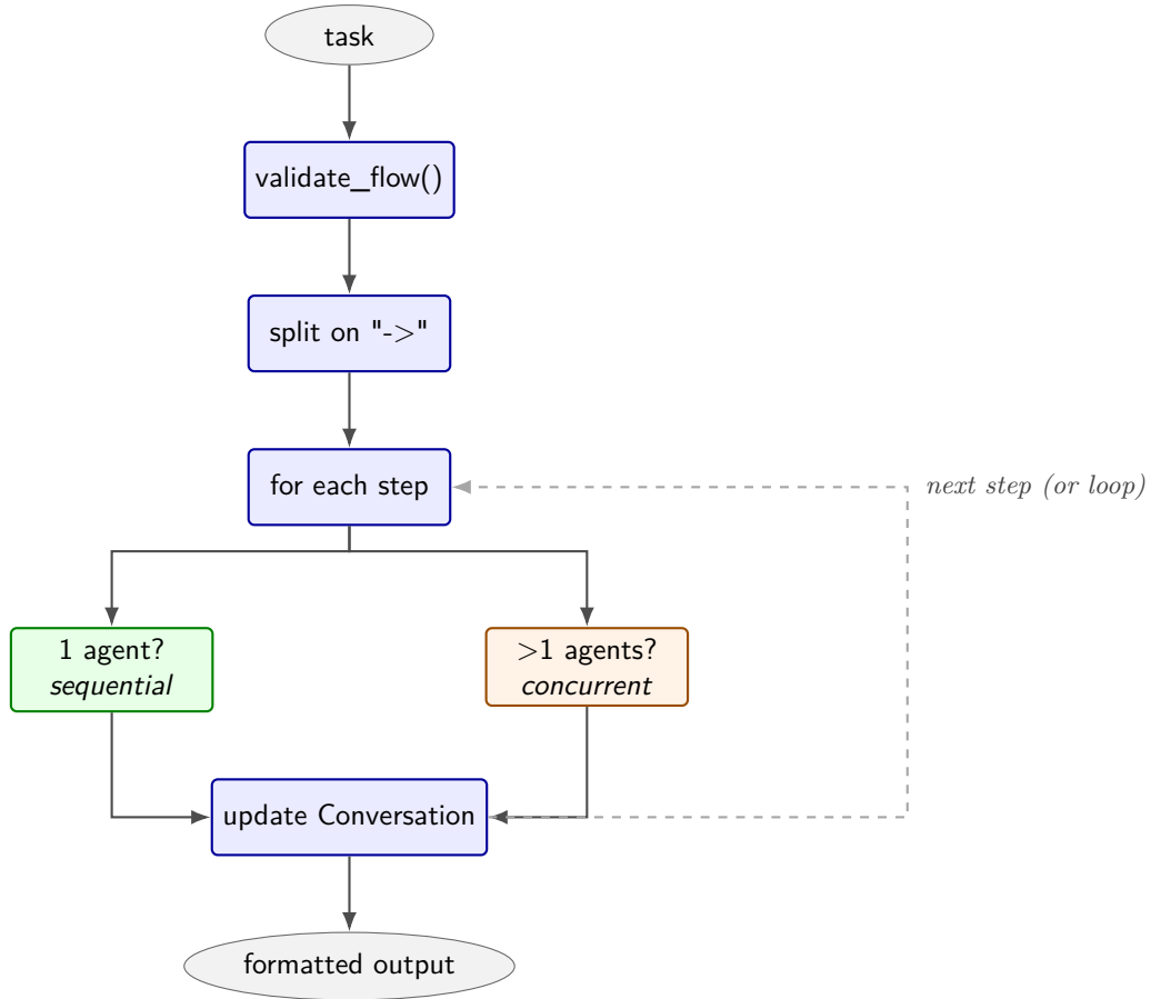
Figure 1: Internal control flow of AgentRearrange._run() .
