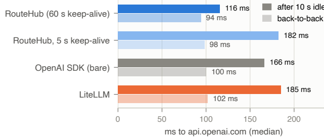
Figure 5: Real network: requests to api.openai.com after a 10s idle gap (solid) and immediately after (light). Medians of 6 repetitions. Only RouteHub’s 60s keep-alive reuses the connection across the gap.
