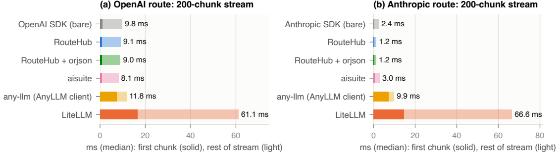
Figure 4: Time to consume a 200-chunk stream from the instant mock server: first content chunk (solid) and the rest of the stream (light), medians of 200 streams. On the Anthropic route every library except the bare SDK also translates each event into an OpenAI chunk.
