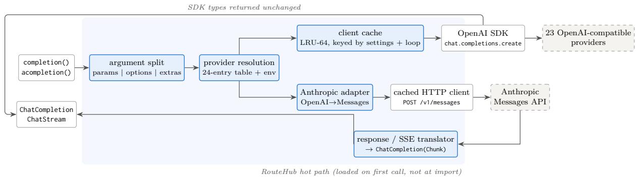
Figure 1: RouteHub request path. Blue boxes are RouteHub code; white boxes are the official OpenAI SDK and HTTP client it delegates to. The OpenAI-compatible path returns the SDK’s own objects; only the Anthropic path translates responses.
