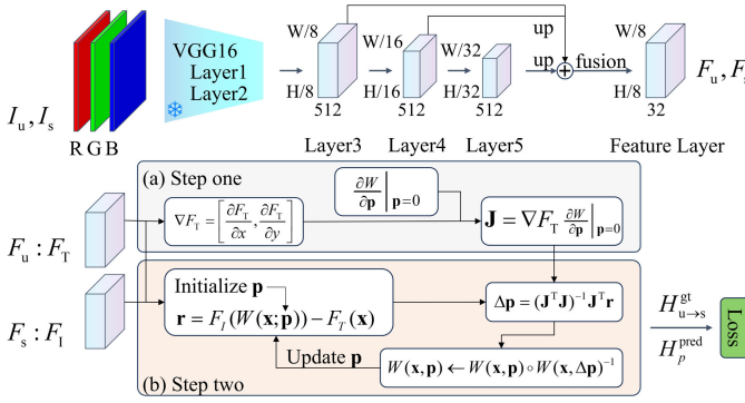
Fig. 4. Schematic of the DLK model. The first two VGG16 blocks are frozen, and features from the last three blocks are fused in an XFeat-style manner. In IC-LK, the satellite image and the UAV image are designated as the input and the template, respectively, which avoids inverting H_{u \rightarrow s}^{\text{gt}} . (a) Step one. (b) Step two.
