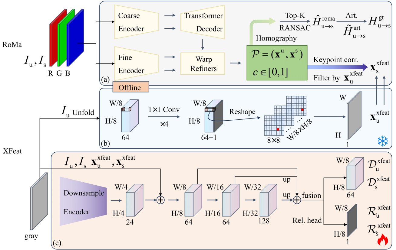
Fig. 3. Data processing and descriptor training. (a) Acquisition of the ground-truth homography H_{u \rightarrow s}^{gt} for I_u and I_s , as well as the sampled correspondence set \mathcal{P} . (b) Keypoint module, which remains frozen during training. (c) Training pipeline for descriptors and reliability maps. Keypoint corr.: Keypoint correspondence and Rel. head: Reliability head.
