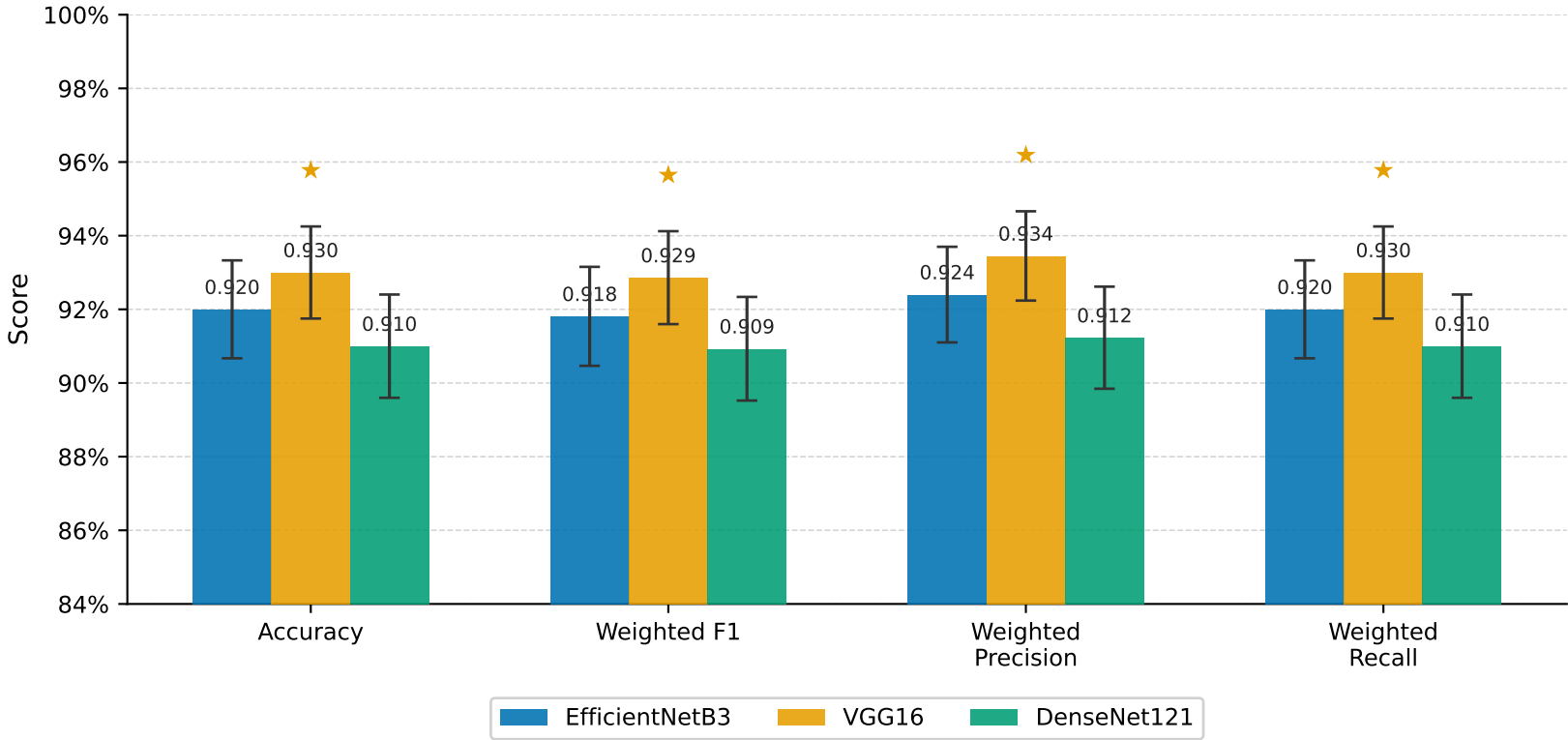
NeuroScan: Overall Model Performance (test set, n = 1,600)
