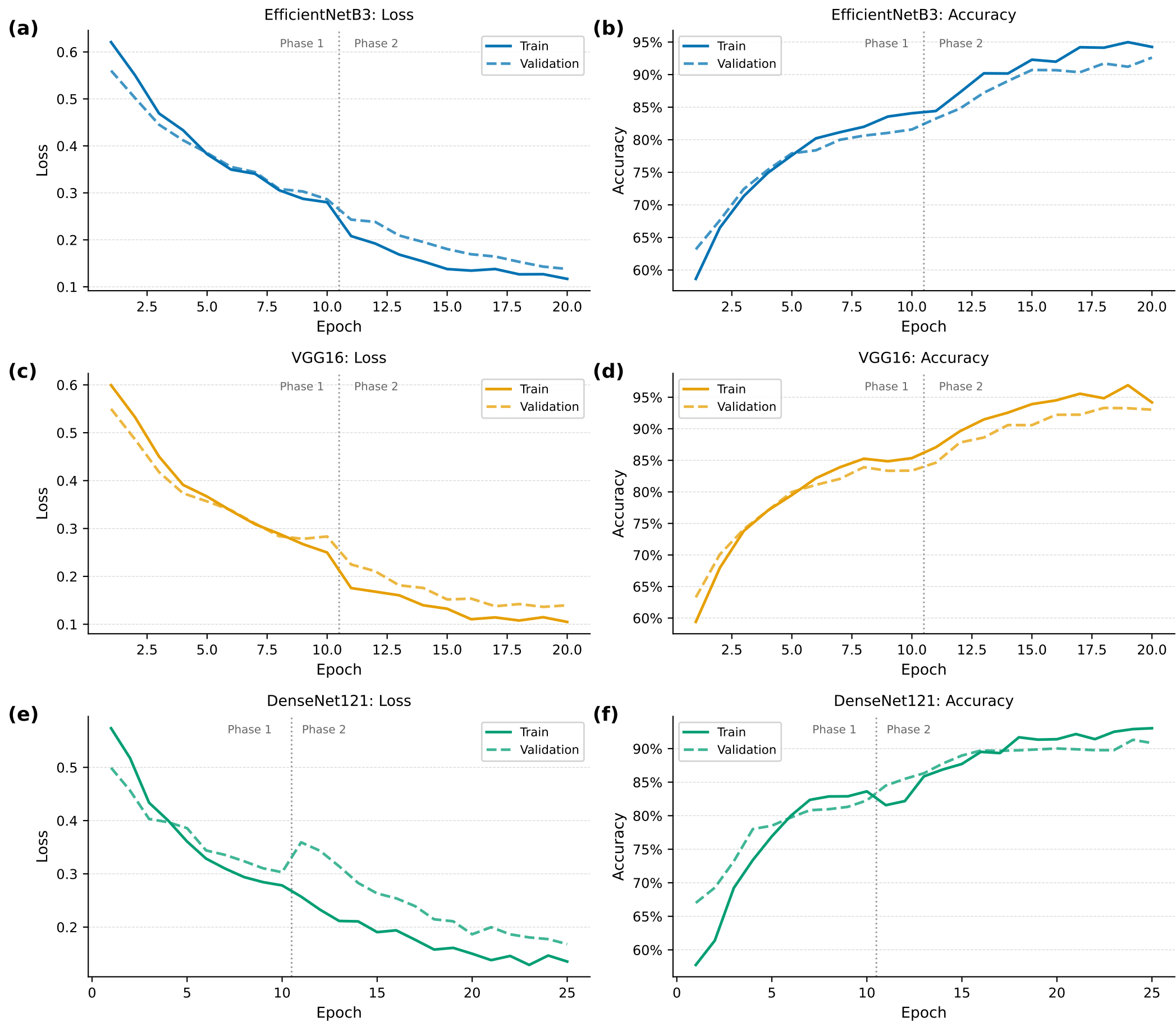
Training Curves: Loss and Accuracy (Phase 1: frozen backbone; Phase 2: fine-tuned)
