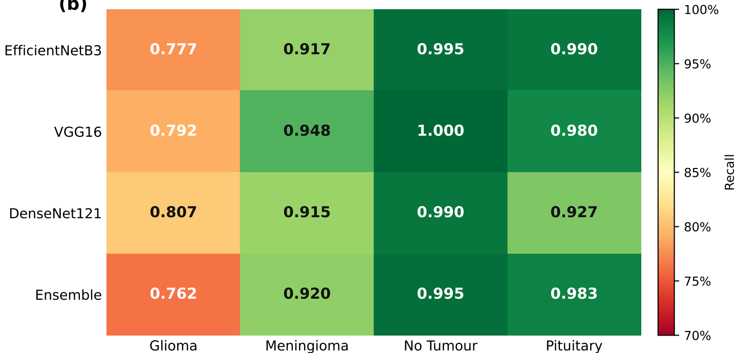
Per-Class Recall: All Models + Ensemble (400 samples / class)
