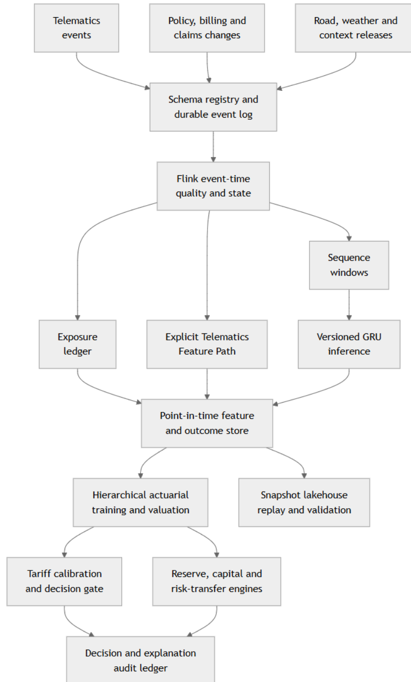
Figure 7. Production architecture preserves event time, point-in-time correctness and model lineage.
