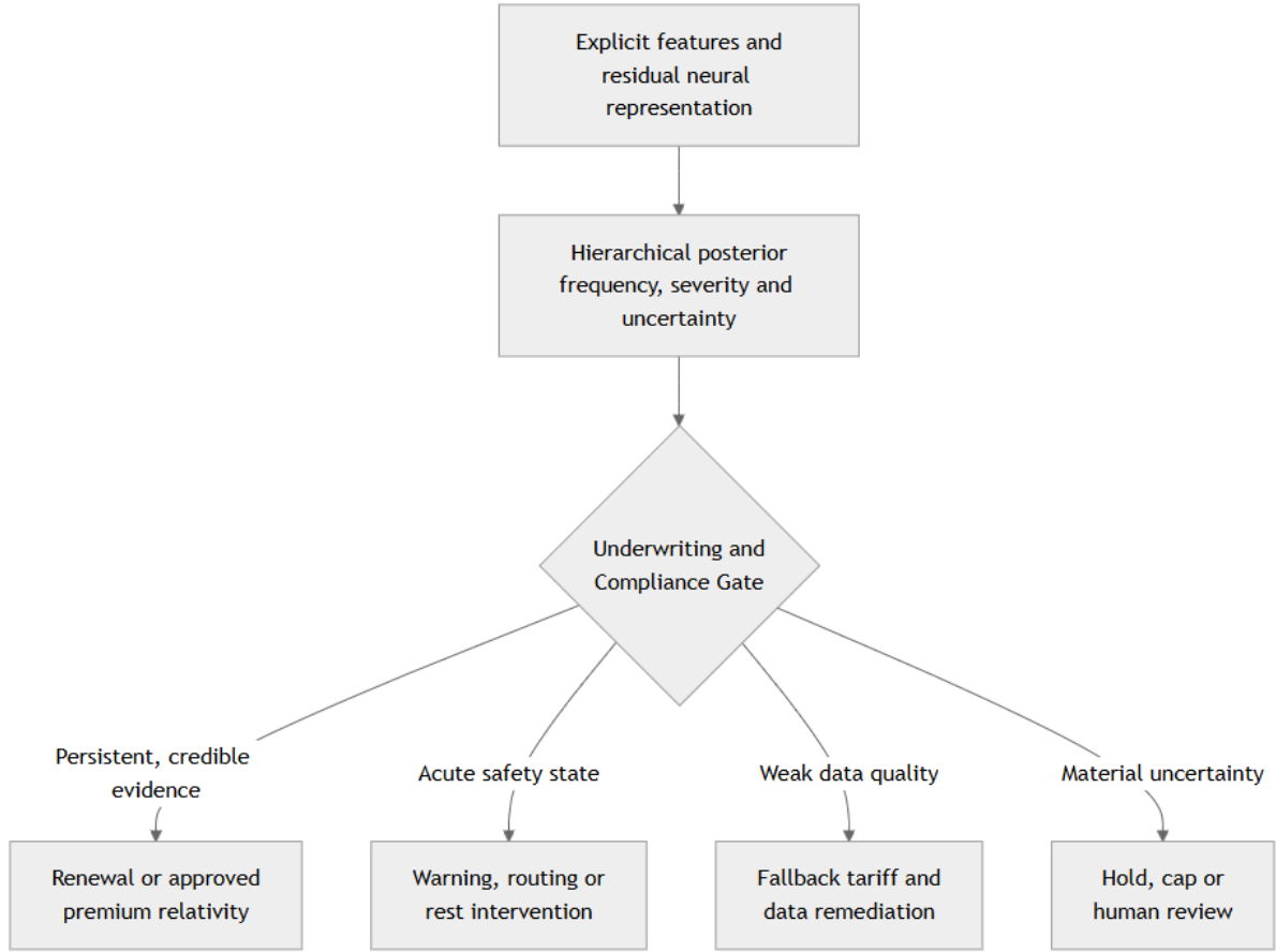
Figure 3. The decision gate separates statistical prediction, tariff action and safety intervention.
