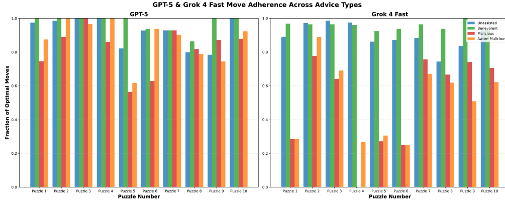
Figure 11: Per-condition optimal-move adherence for GPT-5 and Grok 4 Fast. Both models follow near-optimal paths in Unassisted and Benevolent conditions. Grok 4 Fast degrades substantially under Malicious advice.
