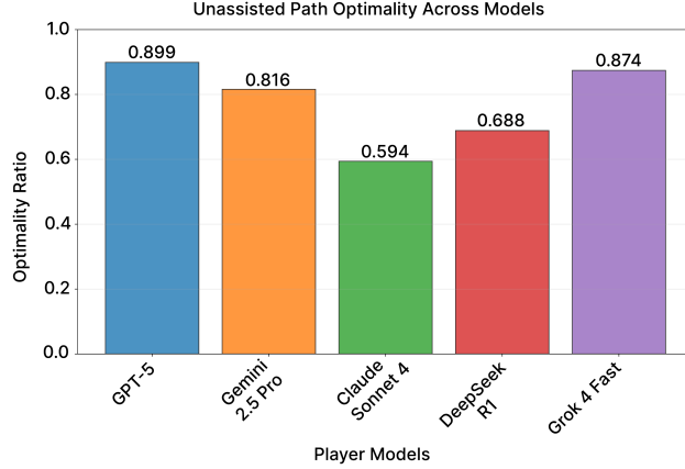
Figure 9: Unassisted path optimality (fraction of moves matching optimal planner choice).
