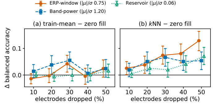
Fig. 3. How much the fill rule alone moves channel-dropout accuracy (feature-coordinate experiment): paired subject-level change in BA relative to zero-fill, with 95% CIs, versus the share of electrodes dropped. (a) Train-mean fill, which differs from zero-fill only by the shift of Eq. (5); the legend gives the mean |\mu|/\sigma of each encoder’s features. (b) kNN fill, which replaces the dropped block by an average of ten training neighbors and so changes its content.
