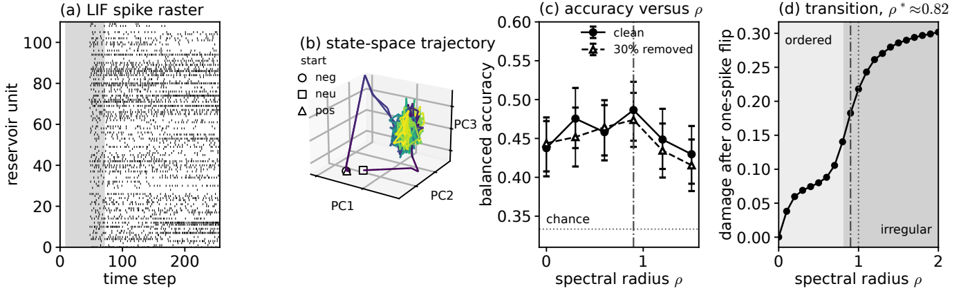
Fig. 1. The fixed LIF reservoir as a dynamical system, linked to accuracy. (a) Spike raster (units 0–109 of 256) for one condition (shaded = the t \in [10, 70] analysis window, about -160 to +73 ms around onset at step 51). (b) Population state-space trajectory (first three principal components of the 256-unit membrane state), colored from epoch start (dark) to end (light), for the three affective conditions; the trajectories largely overlap, consistent with the modest clean separability. (c) Subject-level BA (95% CI) versus spectral radius \rho , clean and with 30% of electrodes removed; \rho = 0 removes the recurrence, and the dash-dot line marks the pre-specified \rho = 0.9 . (d) Damage-spreading order parameter versus \rho ; shading separates the ordered and irregular regimes at the measured transition \rho^* \approx 0.82 ; dash-dot = \rho = 0.9 , dotted = the echo-state heuristic \rho = 1 .
