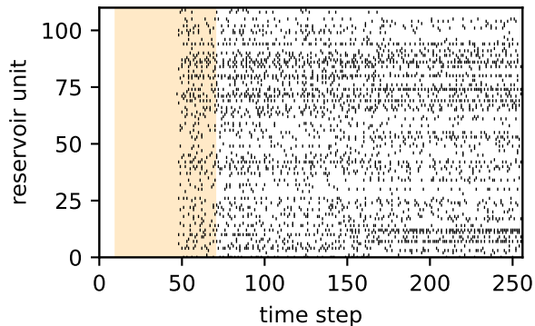
(c) recurrent spectrum ( \rho = 0.9 )
