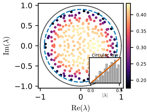
(c) recurrent spectrum ( \rho = 0.9 )
