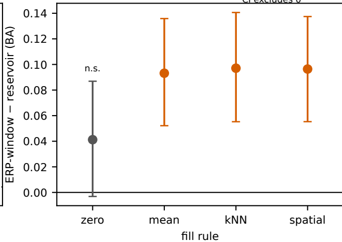
(b) paired subject-level difference at 30% CI excludes 0
