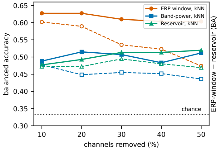
(a) dropout curves: kNN (solid) vs zero (dashed)
