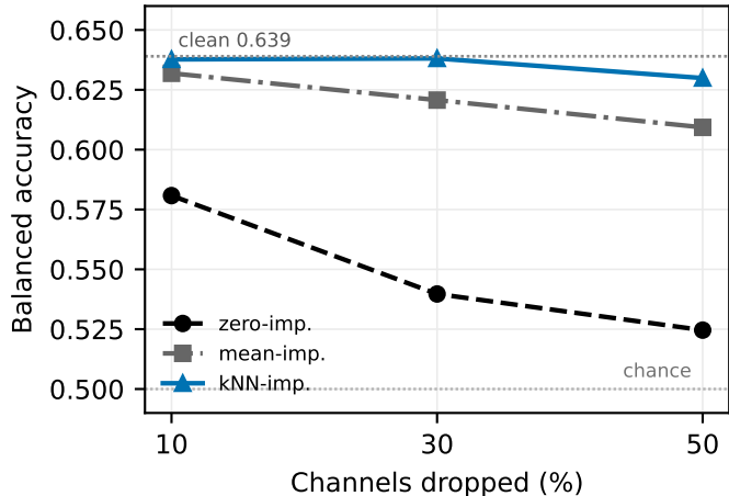
(a) DEAP replication (band-power)
