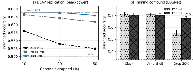
Fig. 4. (a) External check on DEAP [23] (32 subjects, within-subject binary valence, band-power; clean BA 0.639). Channel-dropout BA changes substantially with the imputation rule. (b) EEGNet channel-dropout performance improves from 0.554 to 0.674 when channel-dropout augmentation is used during training, with clean accuracy preserved.
