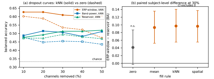
Fig. 3. Subject-level channel-dropout results (feature-coordinate experiment). (a) Balanced accuracy versus channels removed, under k NN fill (solid) and zero fill (dashed). The centered reservoir is nearly flat across fills, whereas ERP-window and band-power gain from the in-distribution fill; k NN-filled ERP-window leads at every rate. (b) Paired subject-level difference ERP-window minus reservoir at 30% dropout, with 95% CIs. The difference is within noise under zero fill and its CI excludes zero under every in-distribution fill, the inference behind Proposition 1.
