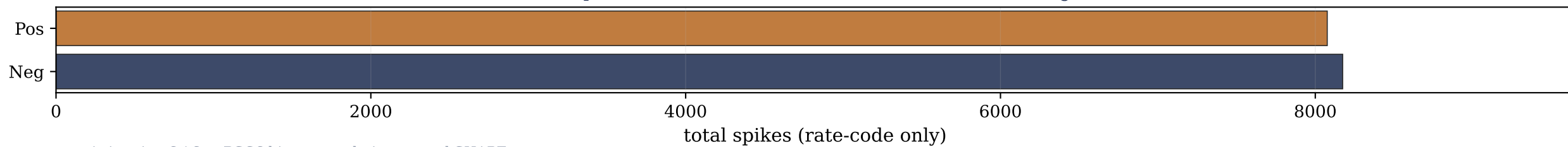
Rate code (total spike count): the two conditions look identical -- timing is what differs
