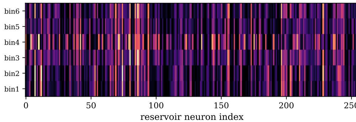
Rate code (total spike count): the two conditions look identical -- timing is what differs
