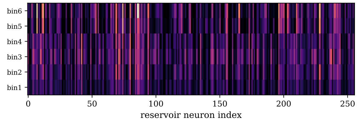
Rate code (total spike count): the two conditions look identical -- timing is what differs
