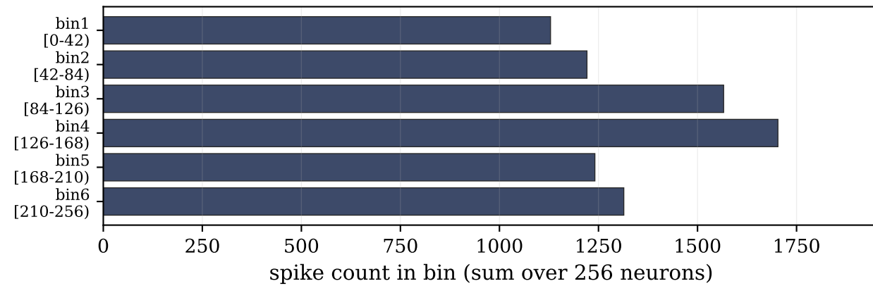
BSC6 feature vector (6 x 256 = 1536-d)
