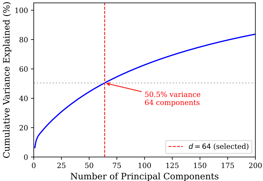
PCA Explained Variance Curve (BSC 6 Features)
