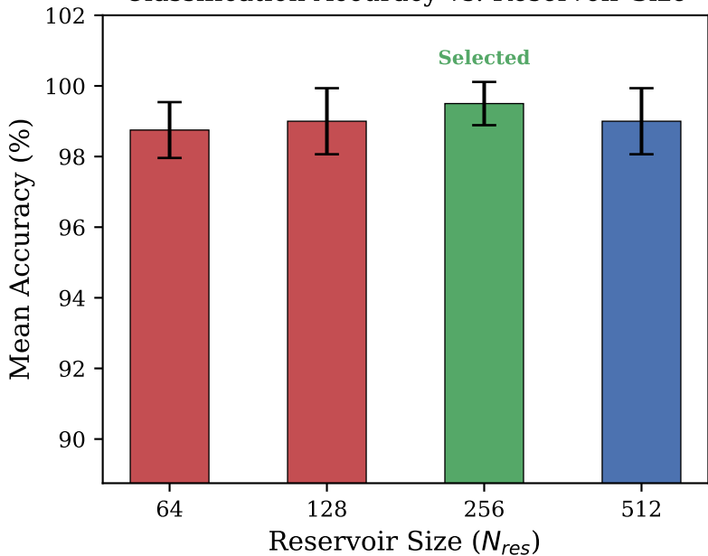
Classification Accuracy vs. Reservoir Size
