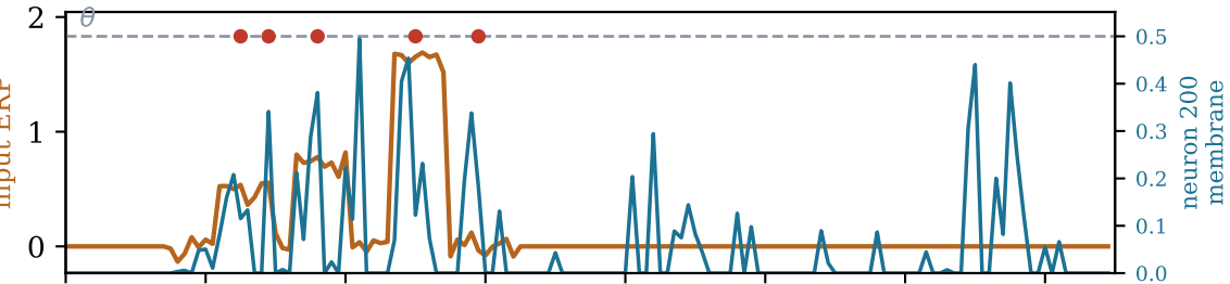
Class 1 - late burst
