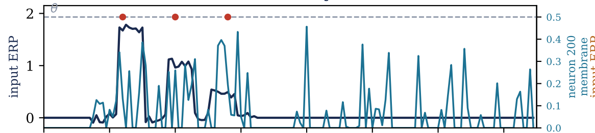
Class 0 - early burst
