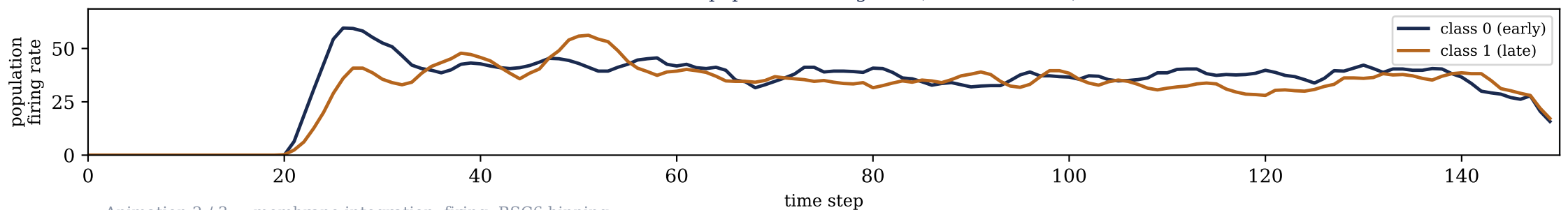
Instantaneous population firing rate (both conditions)
