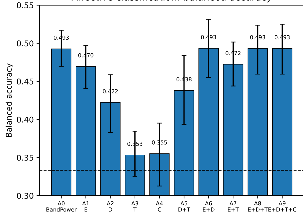
Affective classification: balanced accuracy
