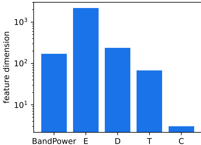
Evidence-stream dimensions
