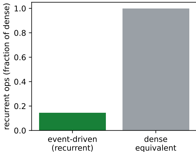
Spike sparsity = 0.14434
