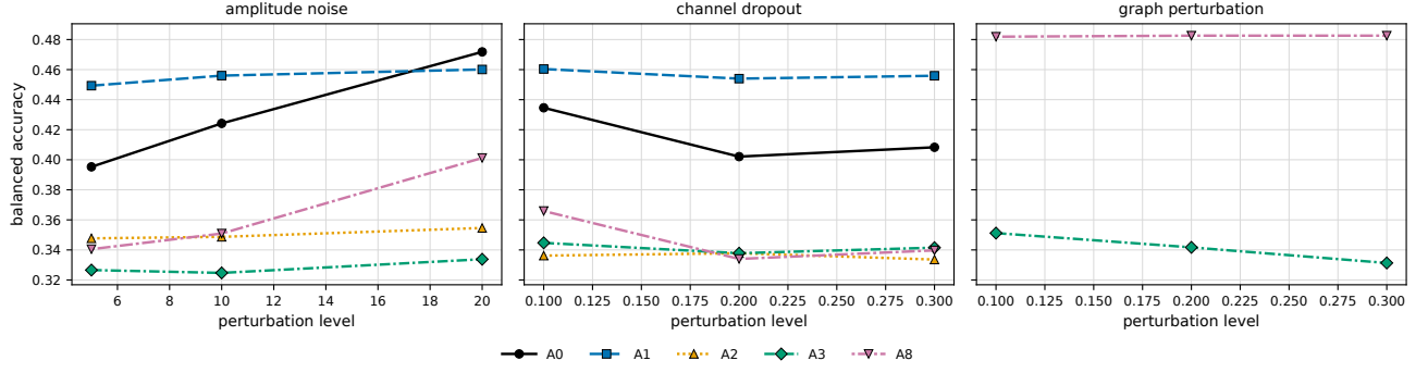
Fig. 5. Representation-level robustness degradation under amplitude noise, channel dropout, and graph edge perturbation for representative configurations. Curves report balanced accuracy as a function of perturbation level; they expose the operating regime of each evidence stream rather than a single endpoint.
