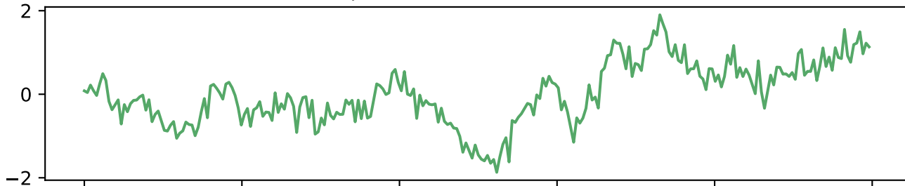
channel dropout (~20%)
