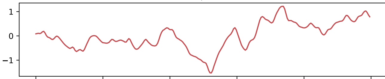
channel dropout (~20%)
