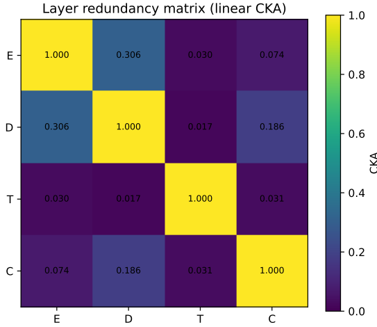
Fig. 3. Representational redundancy across the four evidence streams under linear centered-kernel alignment. The off-diagonal entries are small relative to the unit diagonal, indicating that E , D , T , and C are operationally distinct rather than redundant relabelings of one ERP response.
