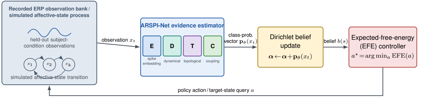
Fig. 5. Neural evidence accumulation over recorded ERP observations. The recorded observation bank emits a held-out subject-condition observation x_t ; the ARSPI-Net evidence estimator updates a Dirichlet belief b(s) over the affective state from the four neural evidence streams; the expected-free-energy controller selects a^* = \arg \min_a \text{EFE}(a) under a risk (pragmatic, toward target) plus ambiguity (epistemic, resolve uncertainty) decomposition and queries the next target affective state until b(\text{target}) \geq 0.8 . Under the simulated affective-state transition the epistemic term adds limited marginal utility, so the controller matches pragmatic-only control. The loop is closed on the belief side and open on the process side.
