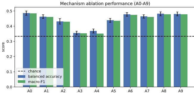
Fig. 3. Mechanism-ablation performance for configurations A0–A9. Balanced accuracy (with bootstrap intervals) and macro-F1 are shown against the three-class chance level. Bars summarise the measured cross-validated performance of each evidence stream and combination.
