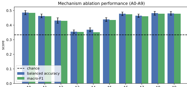
Fig. 3. Mechanism-ablation performance for configurations A0 to A9. Balanced accuracy (with bootstrap intervals) and macro-F1 are shown against the three-class chance level. Bars summarise the measured cross-validated performance of each evidence stream and combination.
