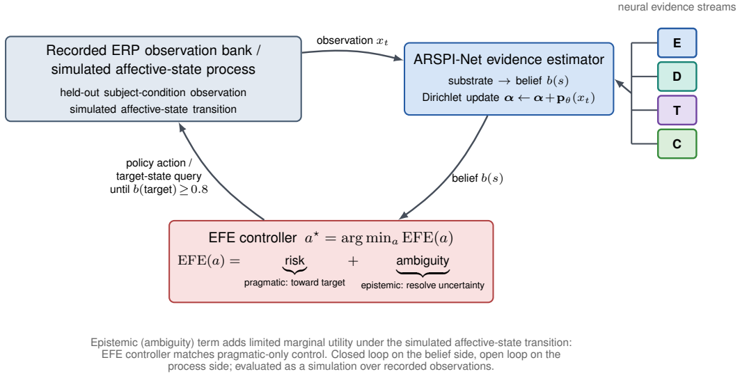
Fig. 5. Neural evidence accumulation over recorded ERP observations. The recorded observation bank emits a held-out subject-condition observation x_t ; the ARSPI-Net evidence estimator updates a Dirichlet belief b(s) over the affective state from the four neural evidence streams; the expected-free-energy controller selects a^* = \arg \min_a \text{EFE}(a) under a risk (pragmatic, toward target) plus ambiguity (epistemic, resolve uncertainty) decomposition and queries the next target affective state until b(\text{target}) \geq 0.8 . Under the simulated affective-state transition the epistemic term adds limited marginal utility, so the controller matches pragmatic-only control. The loop is closed on the belief side and open on the process side.
