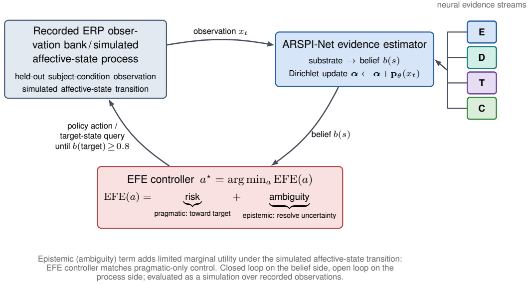
Fig. 5. Neural evidence accumulation over recorded ERP observations. The recorded observation bank emits a held-out subject-condition observation x_t ; the ARSPI-Net evidence estimator updates a Dirichlet belief b(s) over the affective state from the four neural evidence streams; the expected-free-energy controller selects a^* = \arg \min_a \text{EFE}(a) under a risk (pragmatic, toward target) plus ambiguity (epistemic, resolve uncertainty) decomposition and queries the next target affective state until b(\text{target}) \geq 0.8 . Under the simulated affective-state transition the epistemic term adds limited marginal utility, so the controller matches pragmatic-only control. The loop is closed on the belief side and open on the process side.
