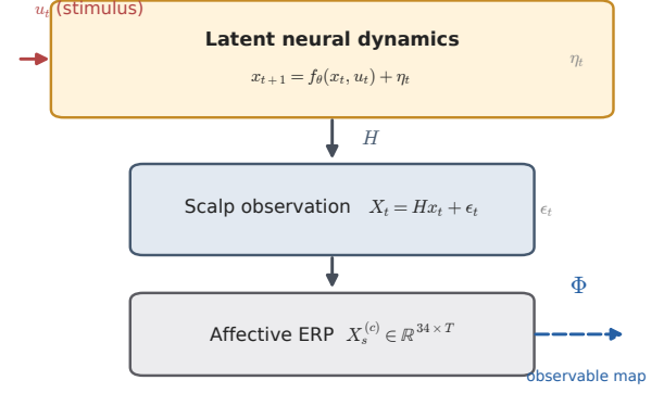
Fig. 2. The affective ERP as the noisy, partially observed output of a latent biological dynamical system. ARSPI-Net’s fixed observable map \Phi reads the recorded scalp observation X_s^{(c)} , not the latent state.
