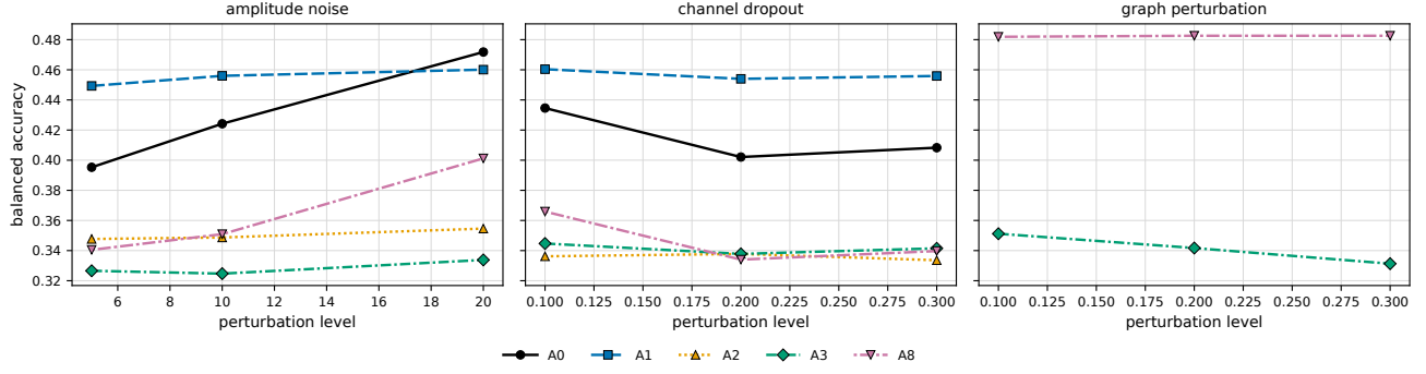
Fig. 7. Representation-level robustness degradation under amplitude noise, channel dropout, and graph edge perturbation for representative configurations. Curves report balanced accuracy as a function of perturbation level; they expose the operating regime of each evidence stream rather than a single endpoint.
