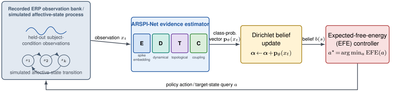
Fig. 8. Neural evidence accumulation over recorded ERP observations. The recorded observation bank emits a held-out subject-condition observation x_t ; the ARSPI-Net evidence estimator updates a Dirichlet belief b(s) over the affective state from the four neural evidence streams; the expected-free-energy controller selects a^* = \arg \min_a \text{EFE}(a) under a risk (pragmatic, toward target) plus ambiguity (epistemic, resolve uncertainty) decomposition and queries the next target affective state until b(\text{target}) \geq 0.8 . Under the simulated affective-state transition the epistemic term adds limited marginal utility, so the controller matches pragmatic-only control. The loop is closed on the belief side and open on the process side.
