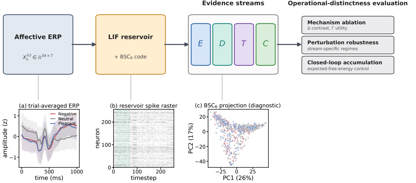
Fig. 1. Overview of ARSPI-Net as a measurement substrate. Each affective ERP observation X_s^{(c)} is transformed by a fixed leaky integrate-and-fire reservoir and a binned spike-count ( BSC_6 ) code into four operationally distinct evidence streams—spike embedding E , dynamical descriptors D , topological descriptors T , and structure-function coupling C —which are then evaluated by mechanism ablation, perturbation robustness, and closed-loop evidence accumulation. Bottom panels are computed from the cohort: (a) trial-averaged ERPs by affective condition, (b) a leaky integrate-and-fire reservoir spike raster for one exemplar observation, and (c) a diagnostic BSC_6 reservoir projection (PCA-2) recomputed from the channel-mean ERP for visual overview only; the production ARSPI-Net spike embedding E used in all reported analyses is defined in Section III.
