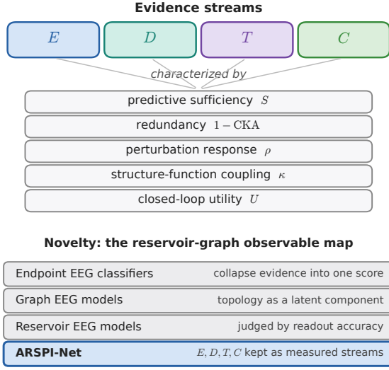
Fig. 3. Operational distinctness. The streams E, D, T, C are characterized by predictive sufficiency, redundancy, perturbation response, coupling, and closed-loop utility. The novelty is the reservoir-graph observable map that keeps the streams separately measurable, unlike endpoint, graph, and reservoir EEG models.
