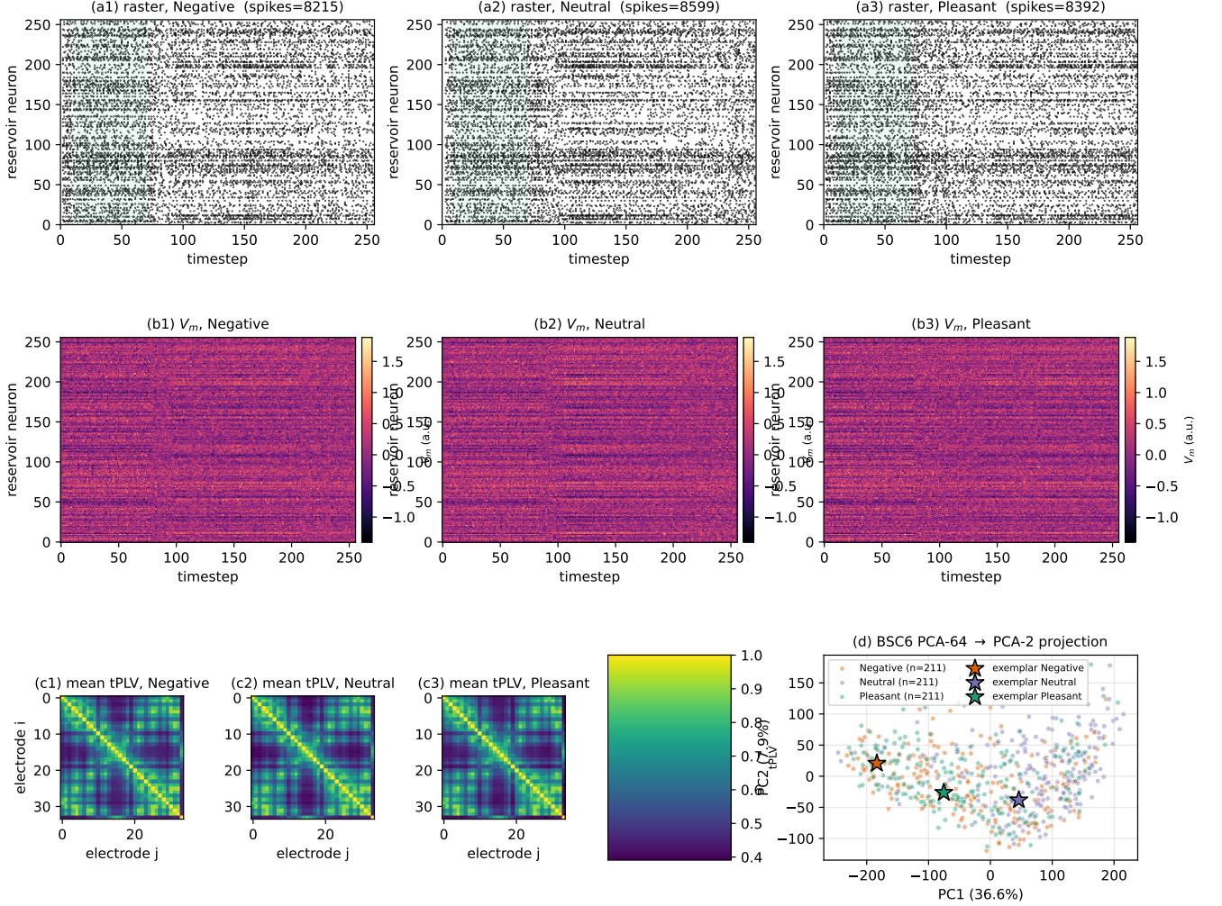
Fig. 5. Computational objects produced by the substrate. (a) LIF spike rasters for one exemplar per affective class on a representative channel; the BSC 6 encoding window t \in [10, 70] is shaded. (b) Membrane-potential heatmaps for the same exemplars. (c) Per-class average 34 \times 34 tPLV connectivity matrices across all 211 subjects. (d) BSC 6 PCA projection (PC1 vs PC2) colored by class with the three exemplars marked.
