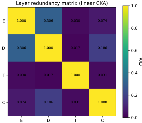
Fig. 6. Representational redundancy across the four evidence streams under linear centered-kernel alignment. The off-diagonal entries are small relative to the unit diagonal, indicating that E , D , T , and C are operationally distinct rather than redundant relabelings of one ERP response.
