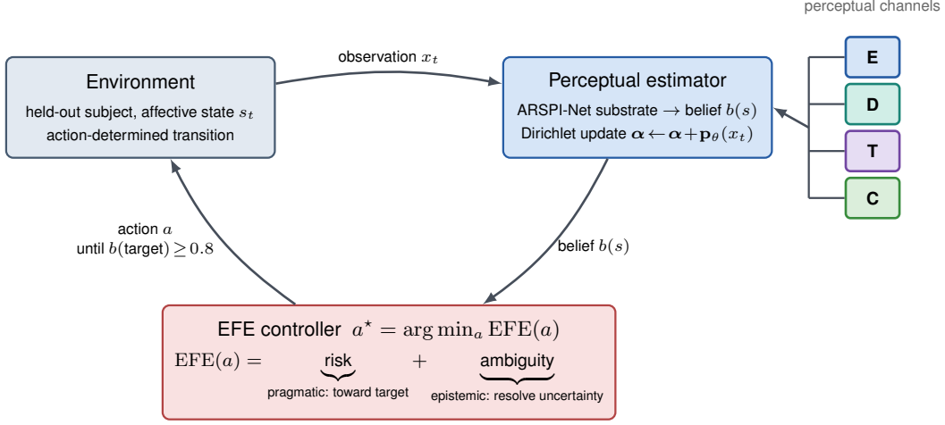
Epistemic (ambiguity) term adds limited marginal utility under action-determined transitions: EFE controller matches pragmatic-only control. Closed loop on the belief side, open loop on the environment side; evaluated as a simulation over recorded observations.
