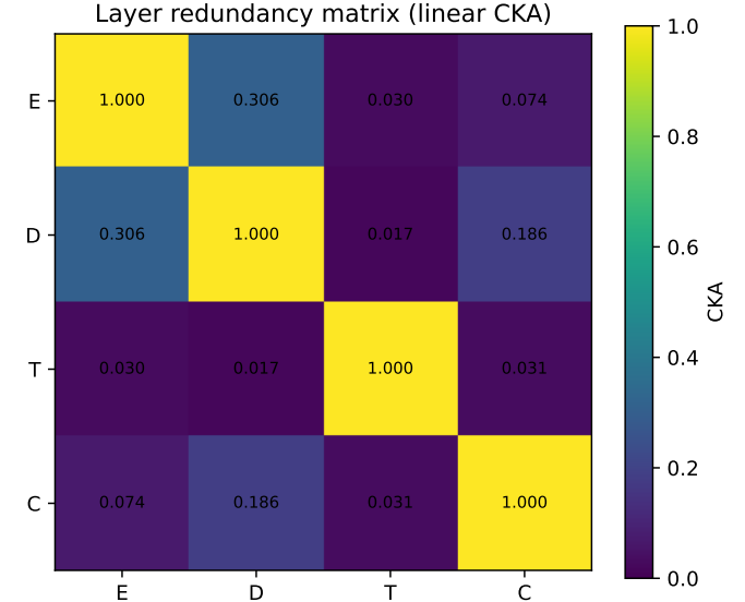
Fig. 7. CKA redundancy matrix. Low-to-moderate values indicate that the feature families are not trivial linear duplicates.
