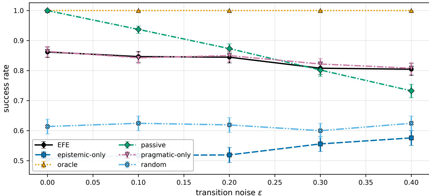
Closed-loop success by policy (Wilson 95% CI)
