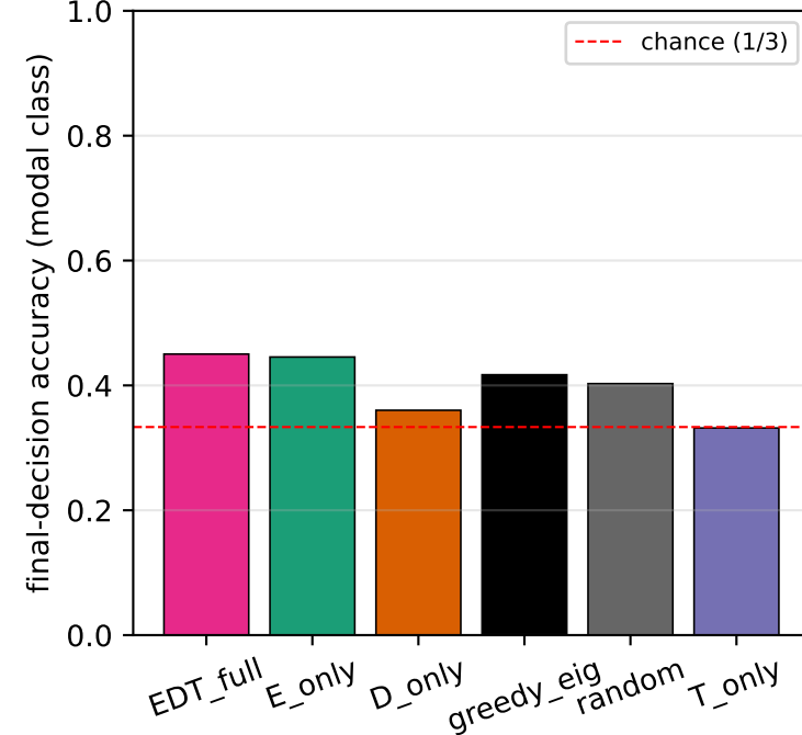
(c) final accuracy after T steps
