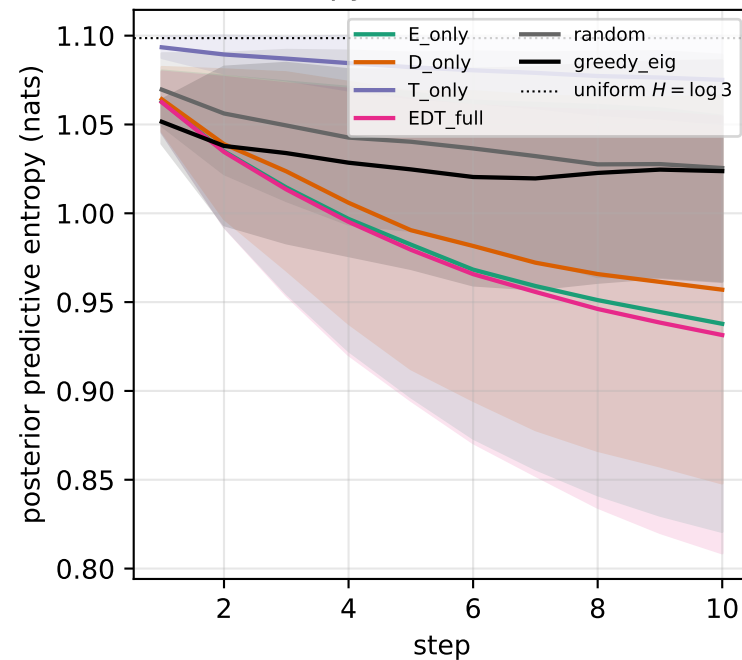
(a) entropy reduction over time
