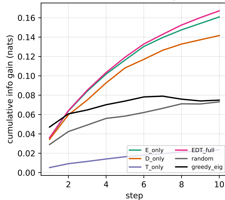
(b) cumulative info gain
