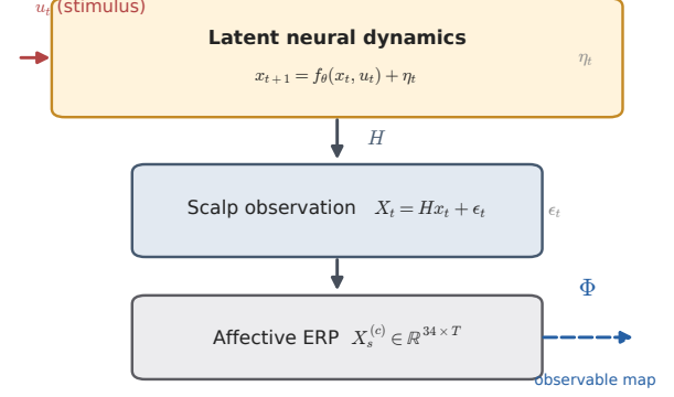
Fig. 2. The affective ERP as the noisy, partially observed output of a latent biological dynamical system. ARSPI-Net’s fixed observable map \Phi reads the recorded scalp observation X_s^{(c)} , not the latent state.
