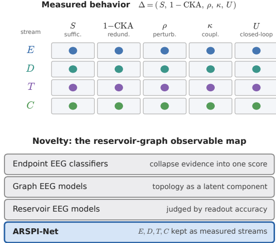
Fig. 3. Operational distinctness. The streams E, D, T, C are characterized by predictive sufficiency, redundancy, perturbation response, coupling, and closed-loop utility. The novelty is the reservoir-graph observable map that keeps the streams separately measurable, unlike endpoint, graph, and reservoir EEG models.
