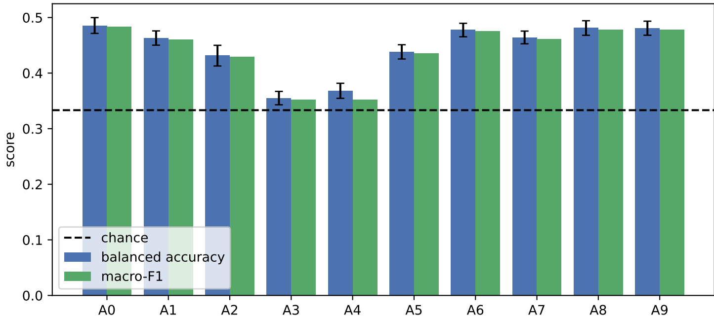
Mechanism ablation performance (A0-A9)
