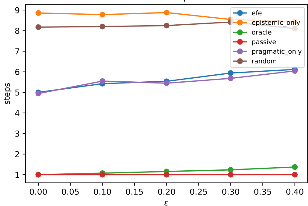
Mean steps
