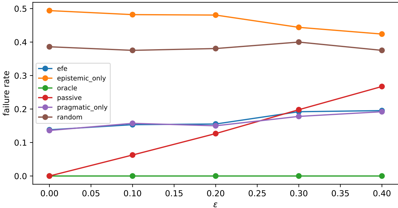
Closed-loop failure rate by policy and transition noise
