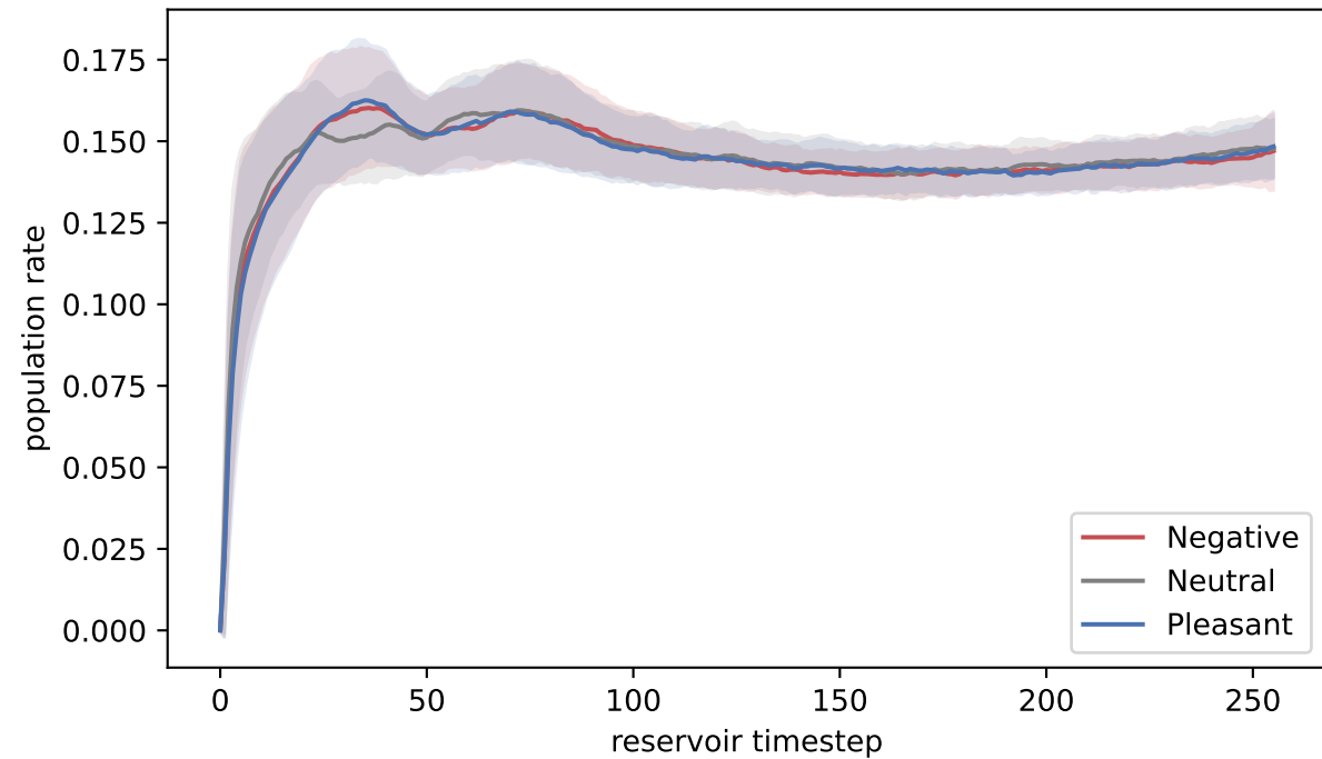
Reservoir population-rate traces by condition
