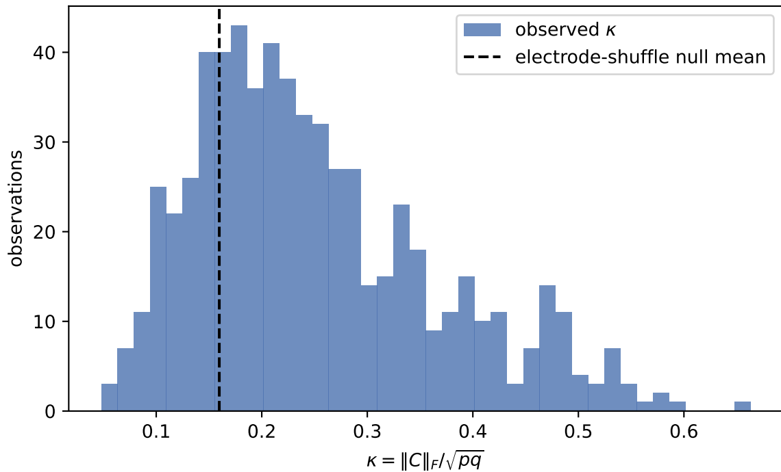
Structure-function coupling \kappa across observations
