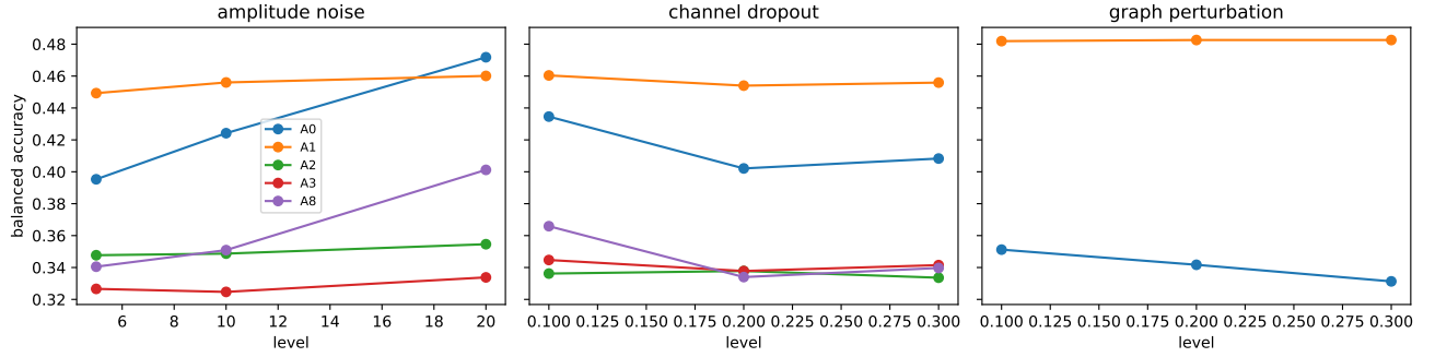
Fig. 14. Representation-level robustness degradation under amplitude noise, channel dropout, and graph edge perturbation for representative configurations. Curves report balanced accuracy as a function of perturbation level; they expose the operating regime of each evidence stream rather than a single endpoint.
