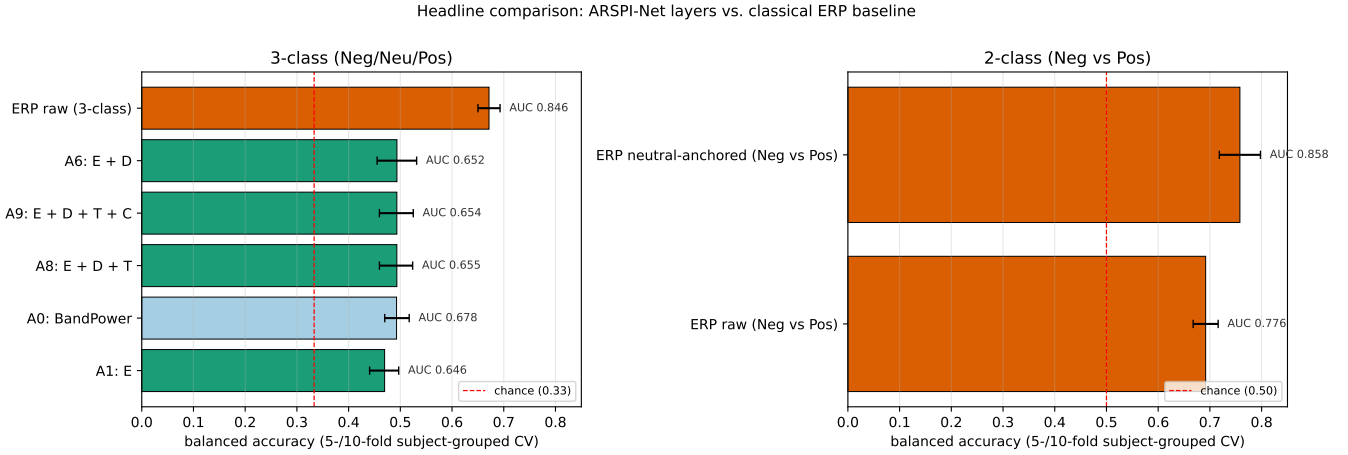
Fig. 11. Headline comparison. ARSPI-Net configurations, the BandPower control, and the classical ERP baseline under matched subject-grouped cross-validation. Numerical AUCs are annotated next to each bar. Chance is marked in red.
