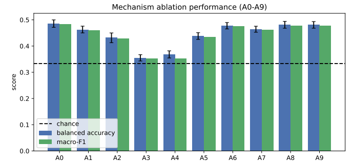
Fig. 13. Mechanism-ablation performance for configurations A0–A9. Balanced accuracy (with bootstrap intervals) and macro-F1 are shown against the three-class chance level. Bars summarise the measured cross-validated performance of each evidence stream and combination.
