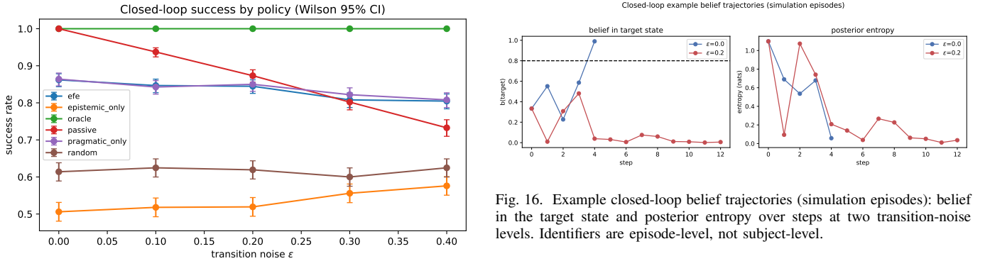
Fig. 15. Closed-loop success rate by policy and transition noise \epsilon , with Wilson 95% intervals. The expected-free-energy and pragmatic controllers reach and confirm the target affective state, while belief-blind, random, and epistemic-only baselines do not.
