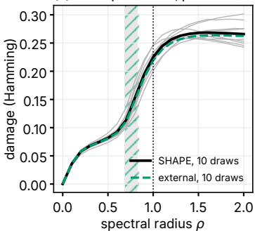
(a) order parameter, \rho^* = 0.76 / 0.76
