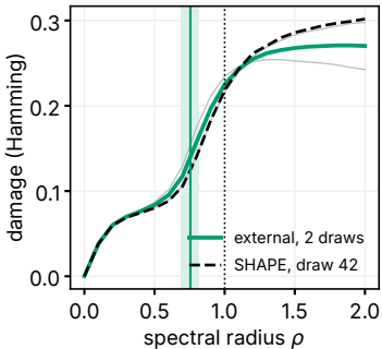
(a) order parameter, \rho^* = 0.76
