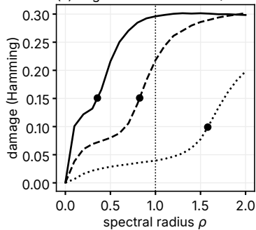
(c) edge versus threshold (SHAPE)
