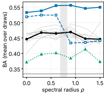
(b) accuracy versus \rho
