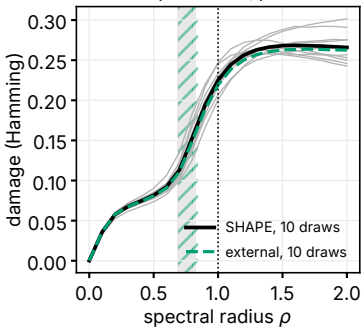
(a) order parameter, \rho^* = 0.76 / 0.76
