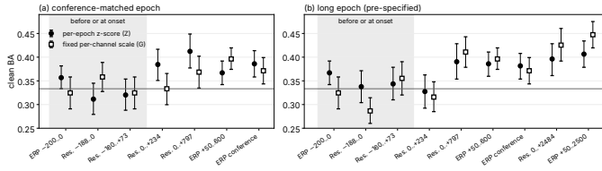
Fig. 6. What each window can read (external cohort, conference-matched epoch). Subject-level BA (95% CI) under per-epoch z-scoring (filled) and a fixed per-channel scale (open), for windows before or at onset (shaded) and after onset. Chance = 1/3 .
