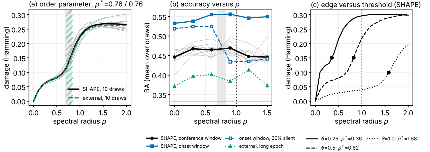
Fig. 7. The measured edge of stability. (a) Damage-spreading order parameter versus spectral radius for ten reservoir draws on SHAPE drives (thin), their mean (thick), and the mean of the same ten draws on the external drives (dashed). The shaded and hatched bands span the transitions \rho^* of the draws on each cohort, and the dotted line marks the echo-state heuristic \rho = 1 . (b) Subject-level BA versus \rho , mean over draws: SHAPE clean with the conference window (thin lines: single draws), with the onset window clean and with 30% of electrodes silent, and with the post window, and the external long epoch (five draws). Shading spans \rho^* of the SHAPE draws. Past it, silent electrodes cost the onset-window code far more accuracy. \rho = 0 removes the recurrence, and chance = 1/3 . (c) Order parameter at three firing thresholds (SHAPE drives, draw 42), with dots at each \rho^* .
