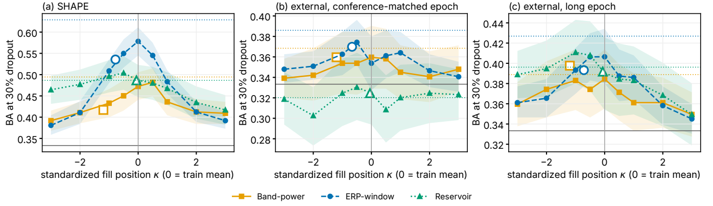
Fig. 5. Moving the fill along the standardized axis (30% of electrodes dropped). Subject-level BA (95% CI, shaded) versus the standardized position \kappa of the filled block ( \kappa = 0 : train-mean fill). Open markers: each encoder's native zero-fill, plotted at minus the mean |\mu|/\sigma of its dropped block for reference (the native zero places each feature at its own -\mu_i/\sigma_i , so it is not a single point on the \kappa axis). Dotted lines: clean BA, which does not depend on the origin (up to solver tolerance). (a) SHAPE: band-power and ERP-window lose as the fill moves away from the training mean in either direction, the reservoir only as it moves above it. (b) External cohort, conference-matched epoch, where every encoder is near chance. (c) External long epoch: the same form at smaller size.
