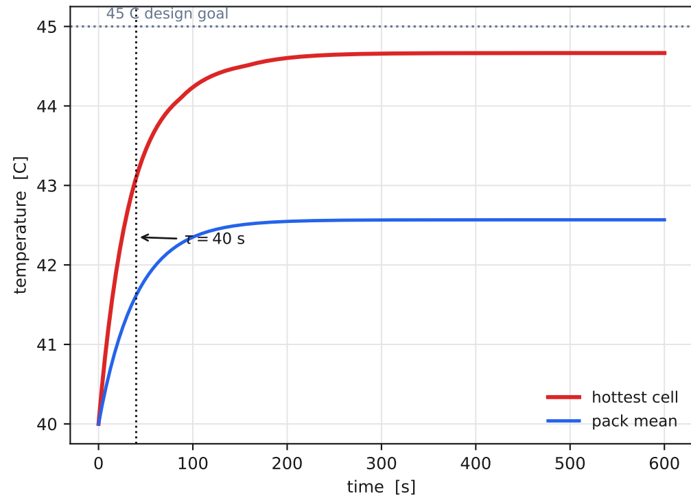
Transient from a cold start
