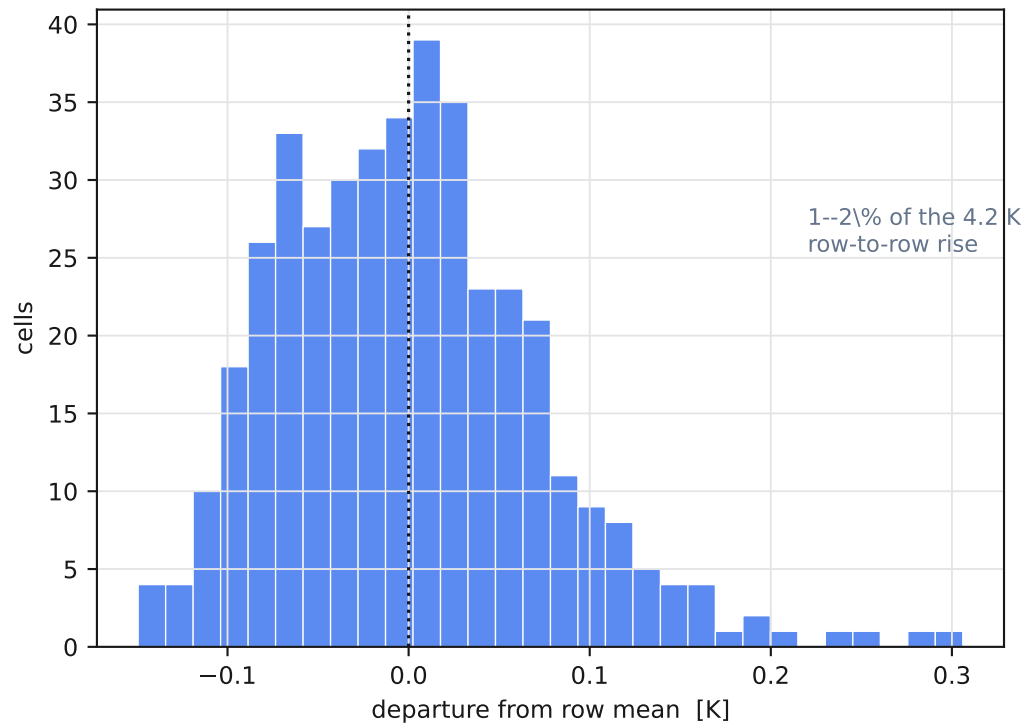
Cell-to-cell scatter ( \sigma_R = 5\% , spread 0.072 K)
