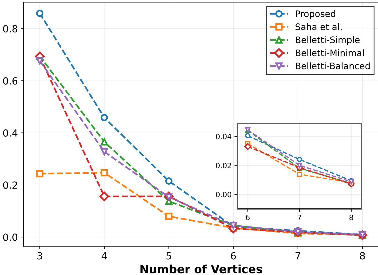
Success Quasi-Probability
